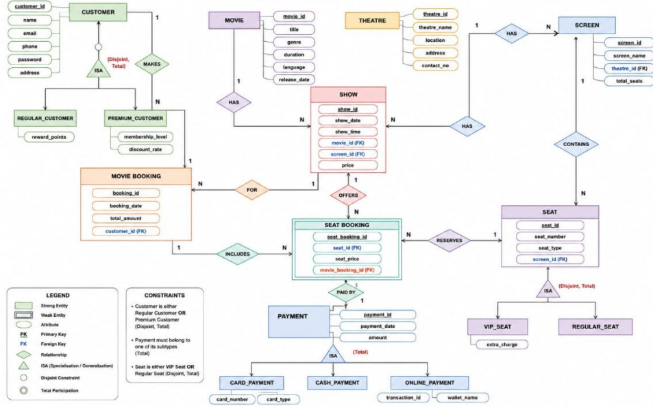
Enhanced Entity Relationship Diagram (EERD) (Movie Booking System)
